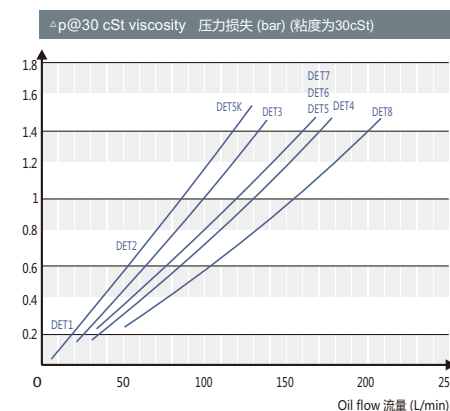
Pressure loss 压力损失 DET1~DET8
